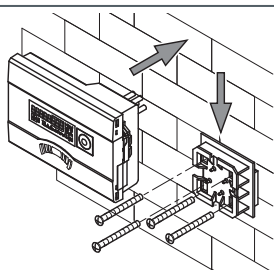
Wall mounting
